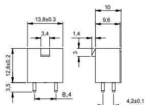
5557S-2*3P针座
